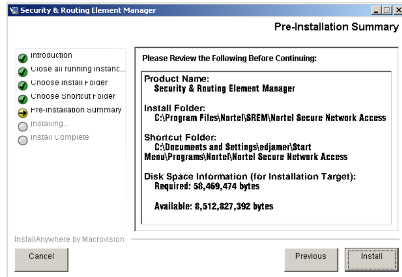
Figure 11 Pre-Installation Summary
